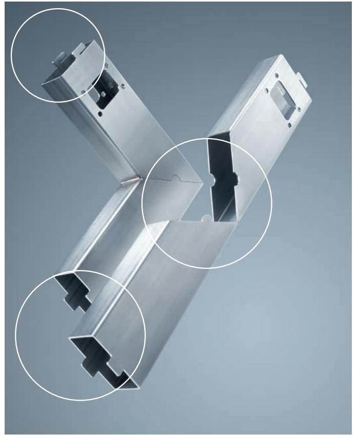
Efficient production of bend connections and positioning aids with a laser.
